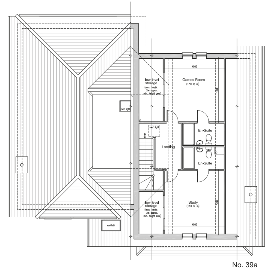
Roof Plan/Second Floor Plan
